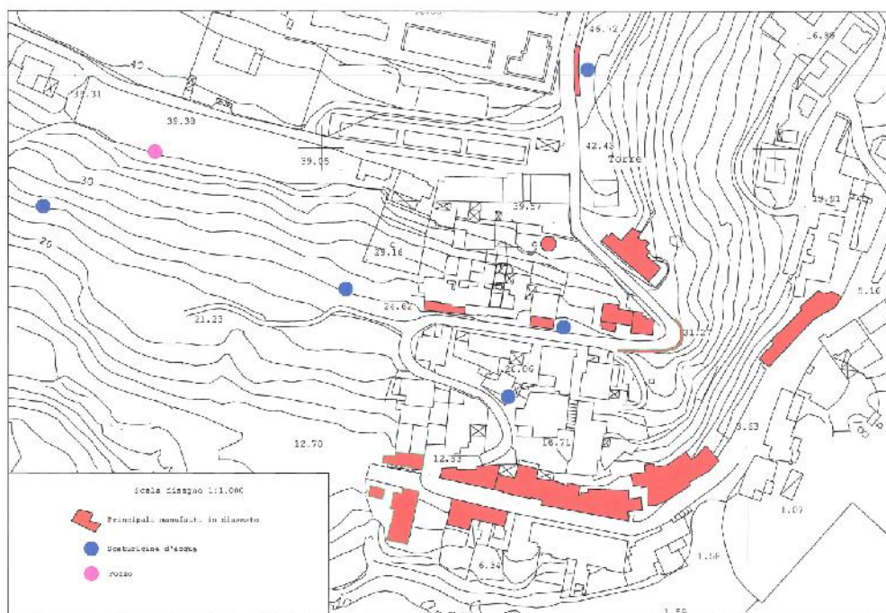
Planimetria fabbricati in dissesto
